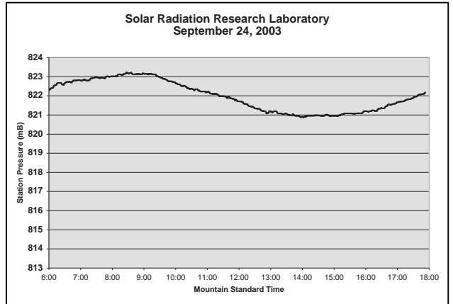
Station Pressure
