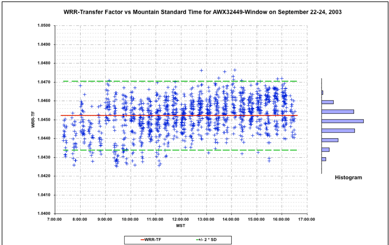
Figure 4.5.13 WRR Transfer Factor vs. Mountain Sdt Time for AHF32449-Window at NPC2003
