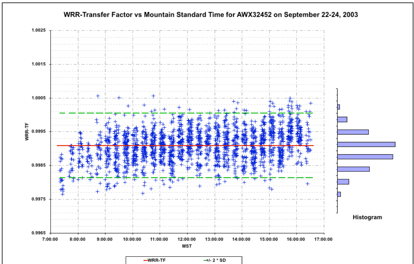
Figure 4.5.14 WRR Transfer Factor vs. Mountain Standard Time for AWX32452 at NPC2003
