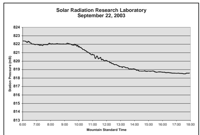
Station Pressure
