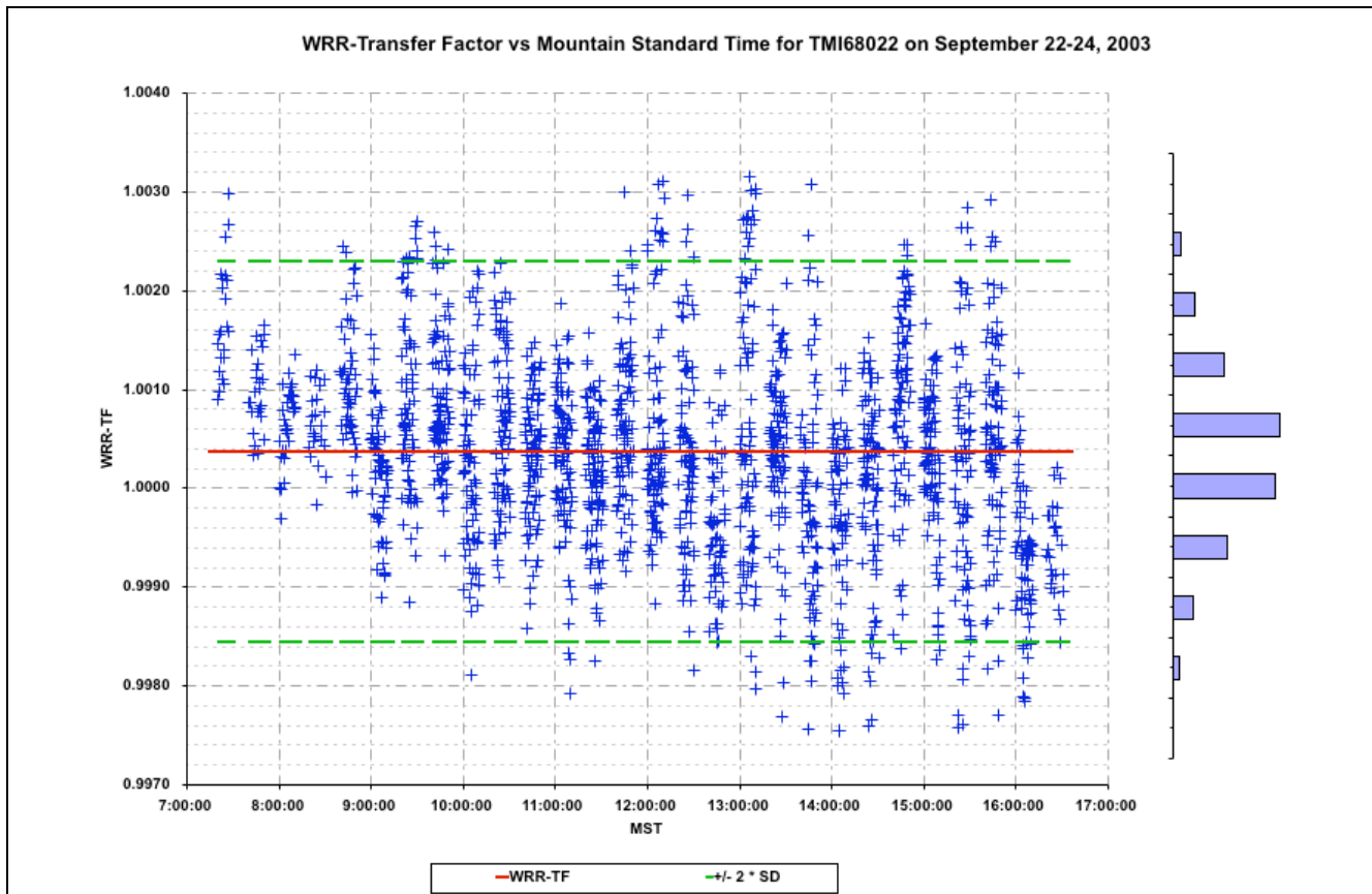
Figure 4.5.19 WRR Transfer Factor vs. Mountain Standard Time for TMI68022 at NPC2003
