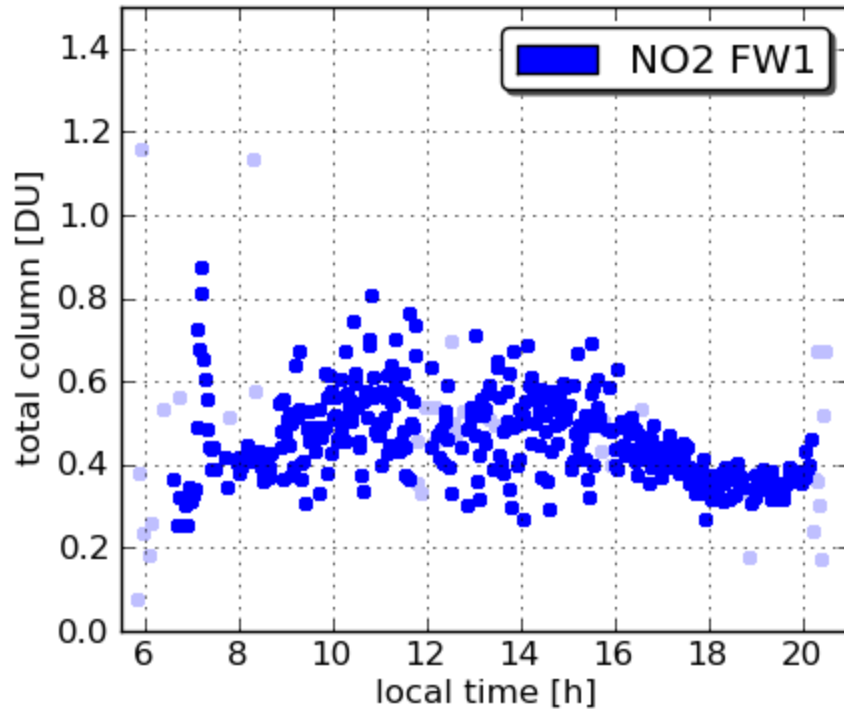
Pandora7 SERC 20110705
