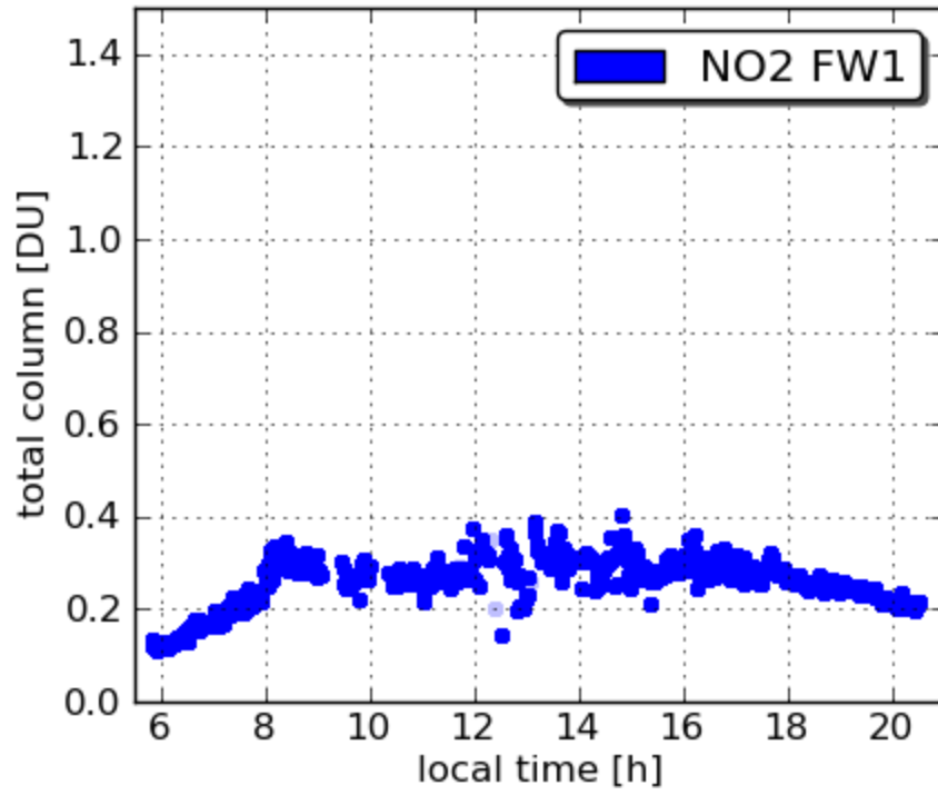
Pandora17 Padonia 20110705
