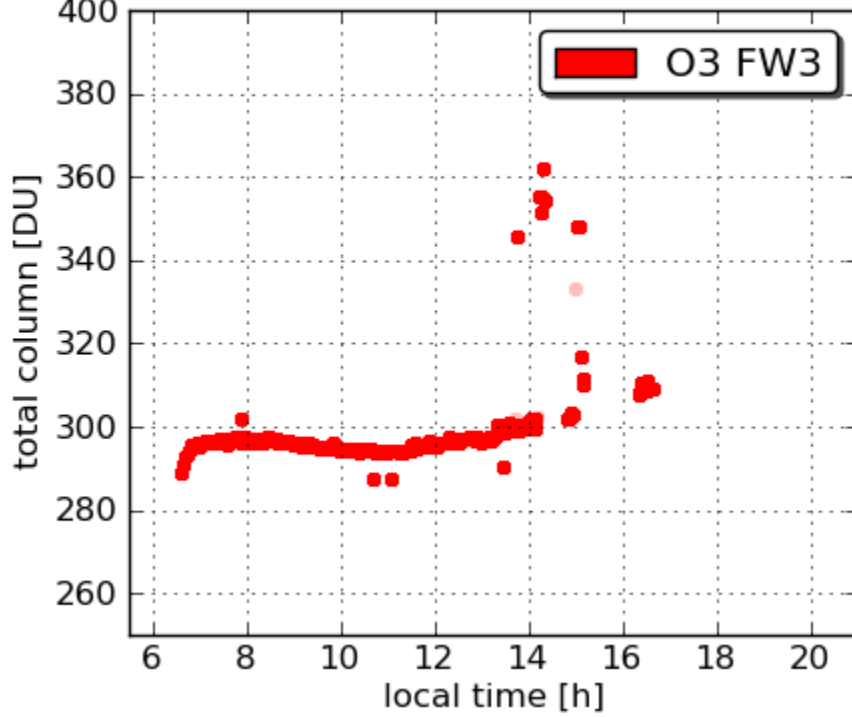
Pandora19 Essex 20110705
