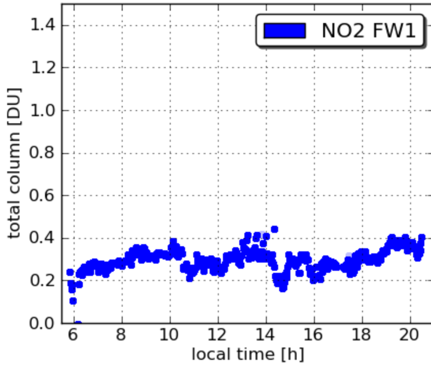
Pandora3 GSFC 20110704
