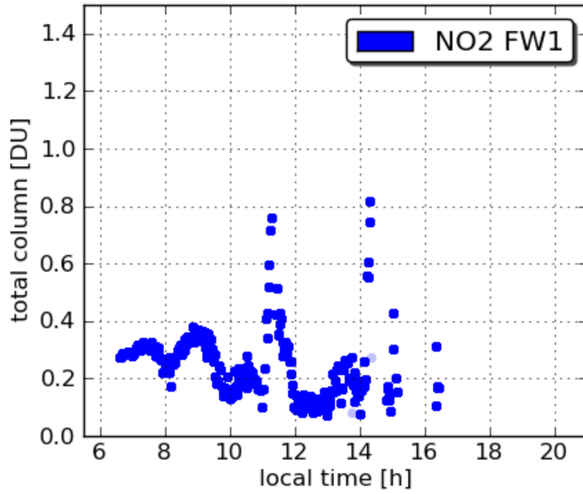
Pandora19 Essex 20110705
