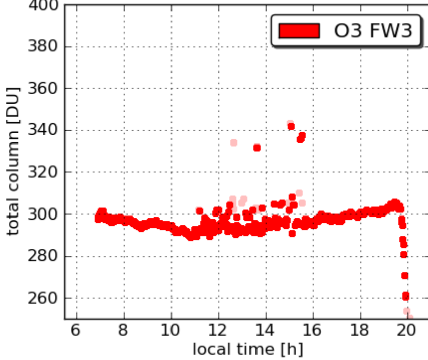
Pandora20 Beltsville 20110705
