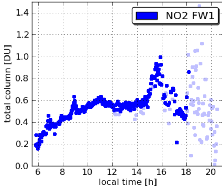
Pandora18 Edgewood 20110705
