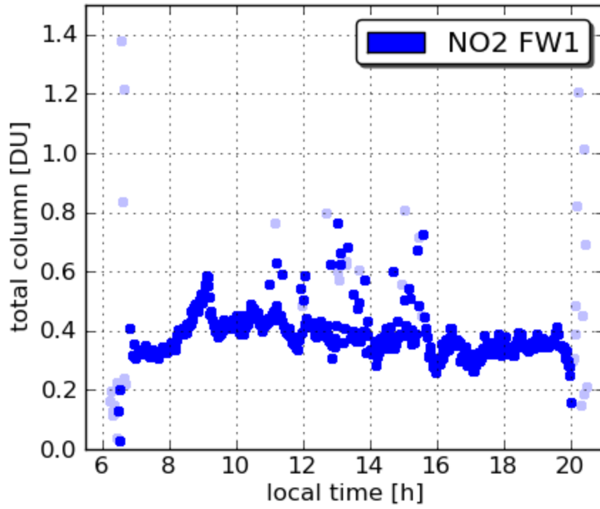
Pandora20 Beltsville 20110705
