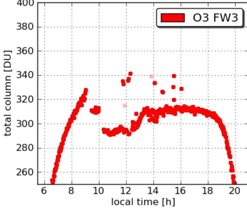
Pandora17 Padonia 20110705
