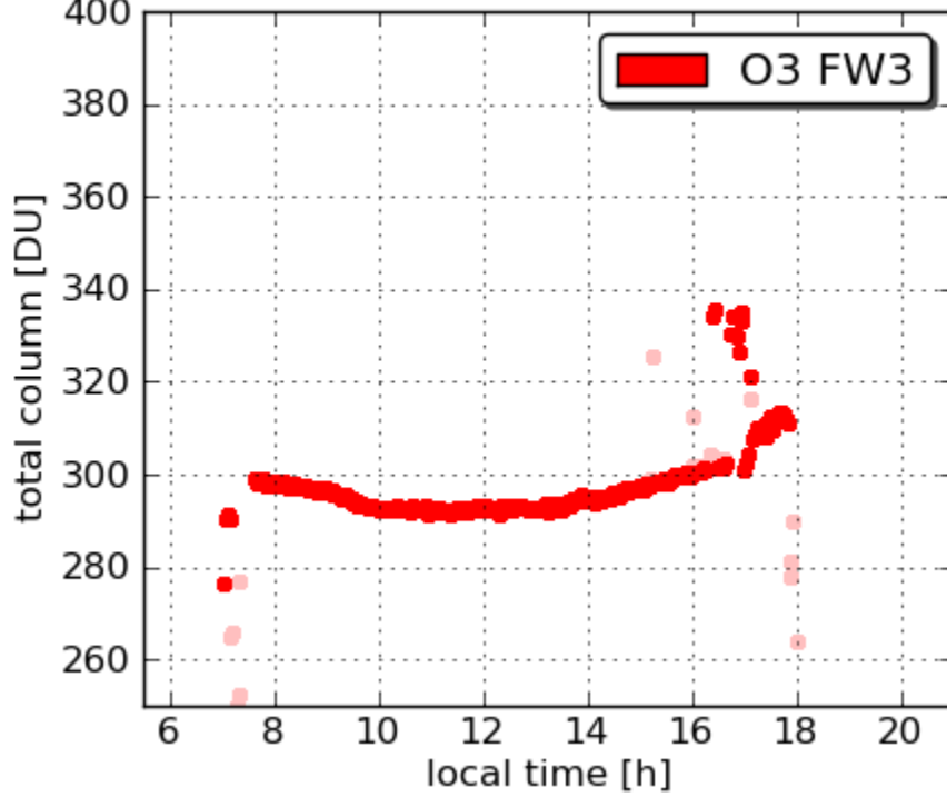
Pandora18 Edgewood 20110705
