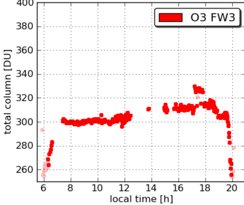
Pandora23 Aldino 20110705
