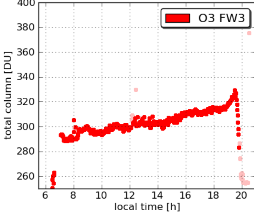
Pandora16 Fairhill 20110705
