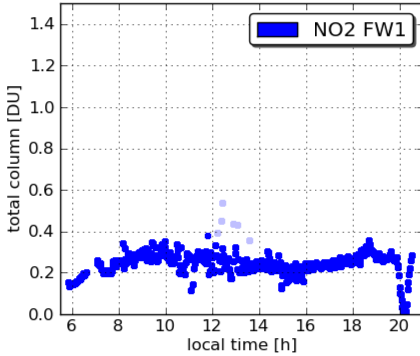
Pandora16 Fairhill 20110705
