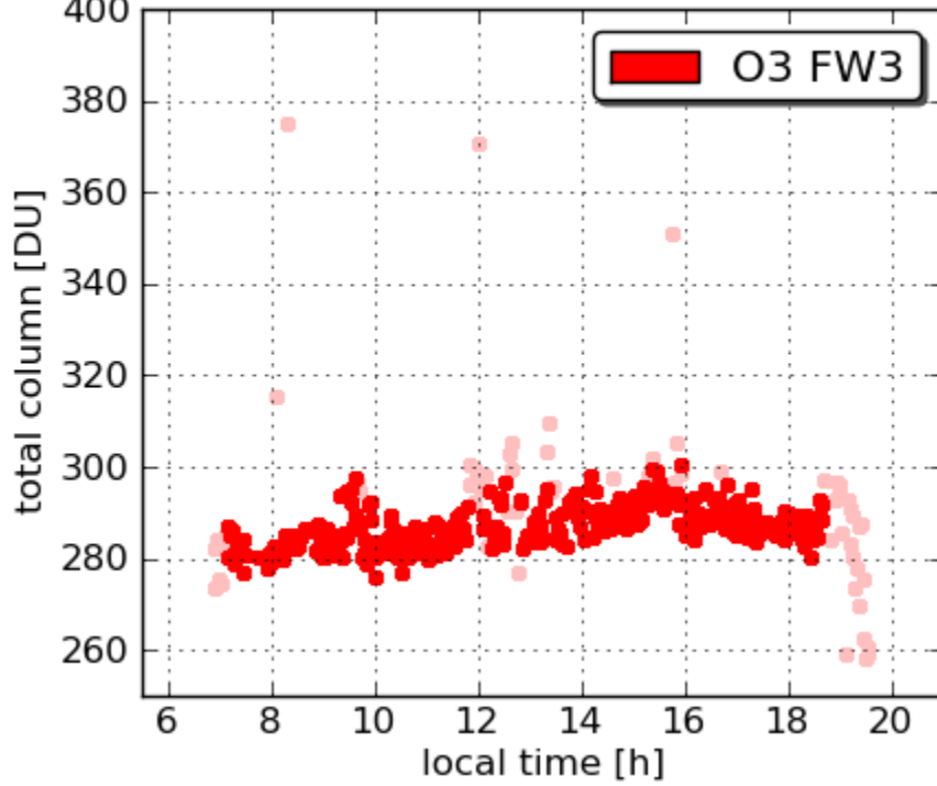
Pandora7 SERC 20110705
