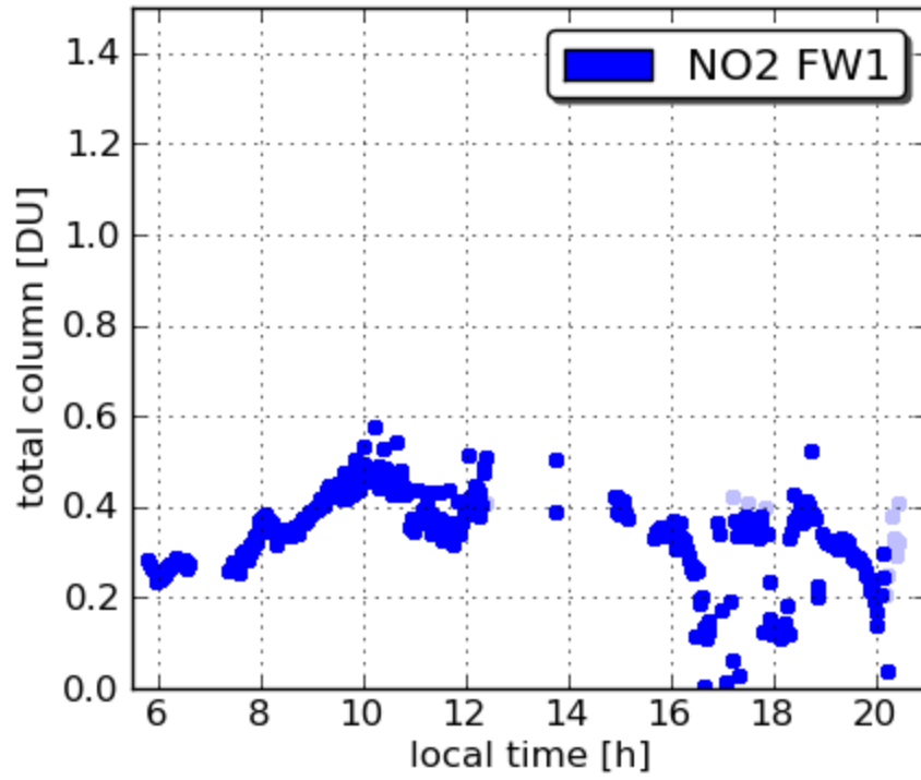
Pandora23 Aldino 20110705
