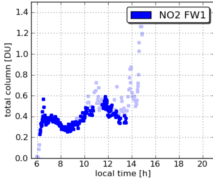
Pandora3 GSFC 20110713
