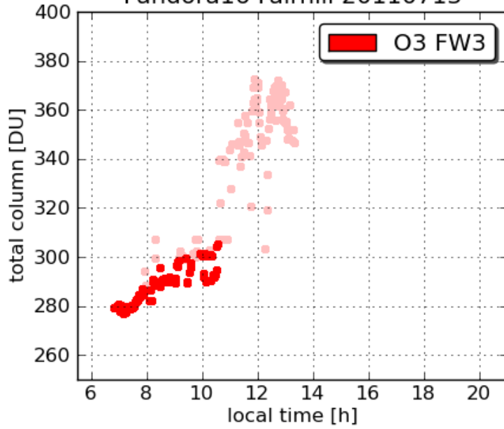
Pandora16 Fairhill 20110713
