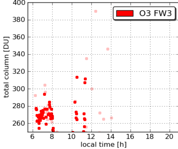
Pandora9 Oldtown 20110713
