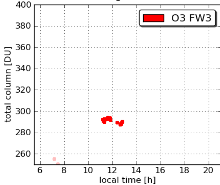
Pandora18 Edgewood 20110713
