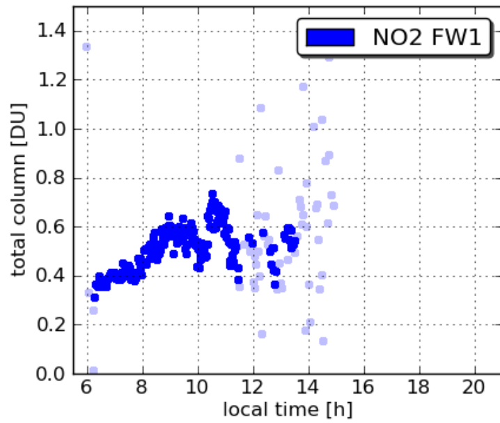
Pandora9 Oldtown 20110713
