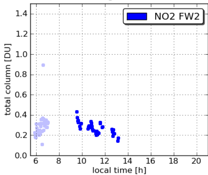
Pandora18 Edgewood 20110713
