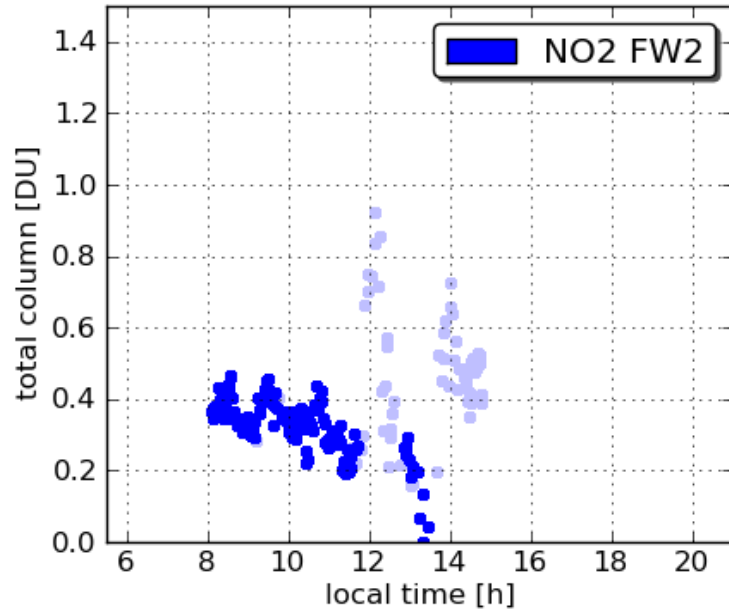
Pandora19 Essex 20110713
