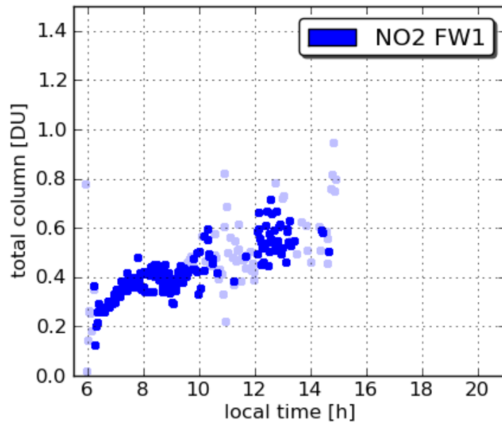
Pandora7 SERC 20110713
