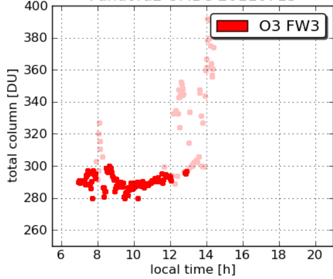
Pandora2 UMBC 20110713
