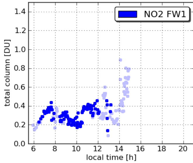
Pandora2 UMBC 20110713
