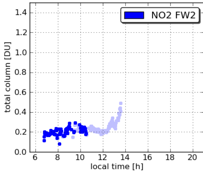
Pandora16 Fairhill 20110713
