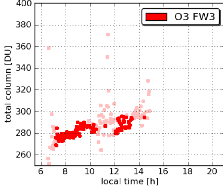
Pandora7 SERC 20110713
