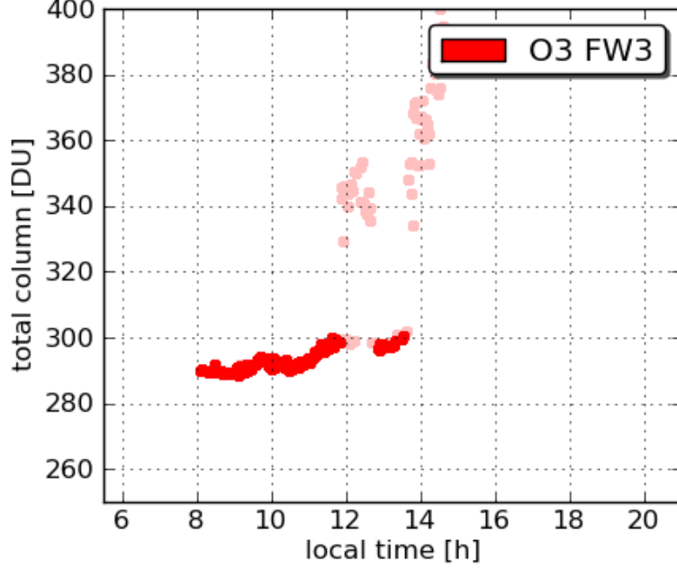
Pandora19 Essex 20110713
