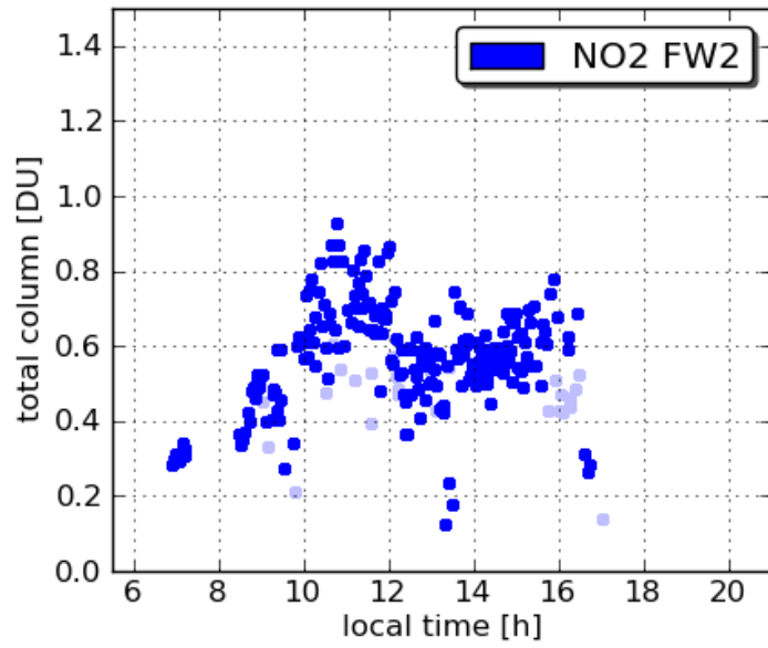
Pandora24 Chesapeakebay 20110718
