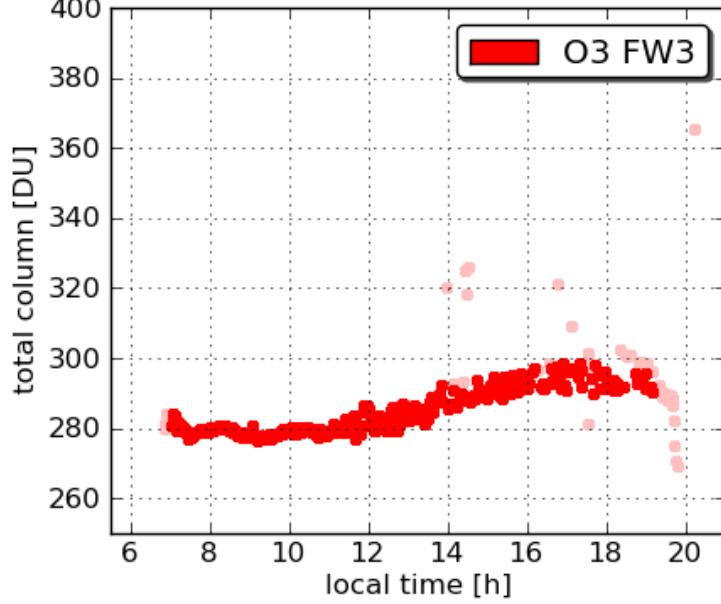
Pandora20 Beltsville 20110718
