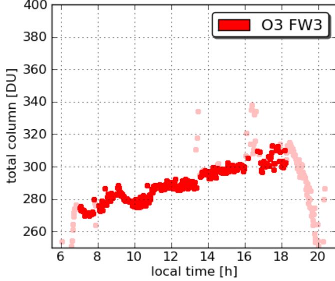
Pandora16 Fairhill 20110718
