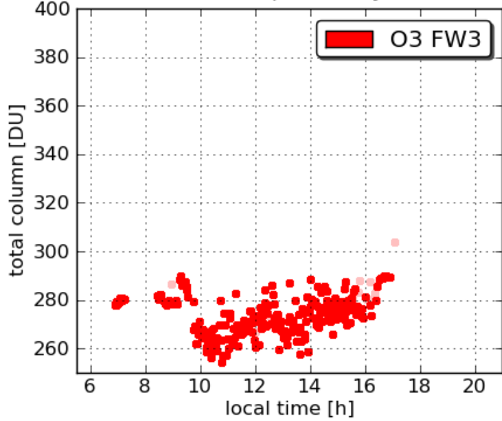
Pandora24 Chesapeakebay 20110718
