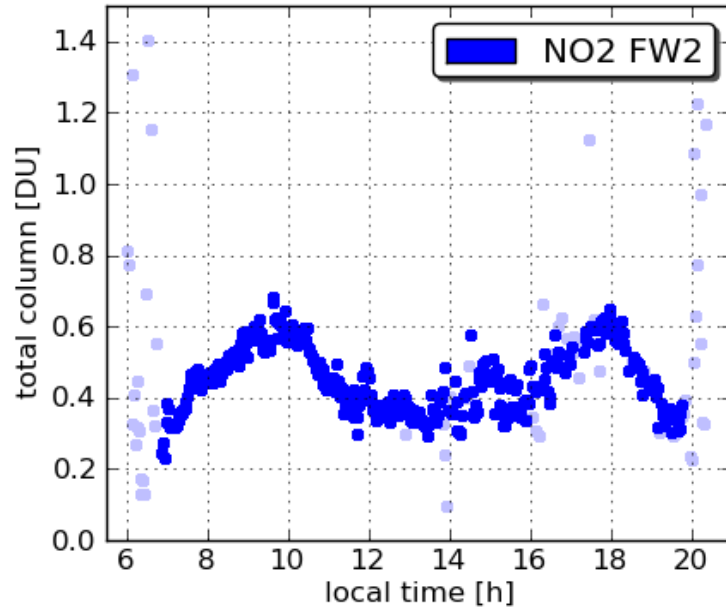
Pandora20 Beltsville 20110718
