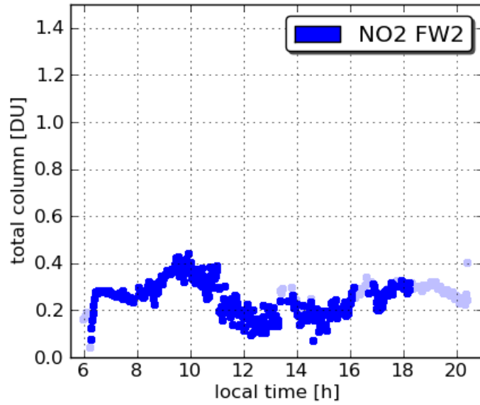
Pandora16 Fairhill 20110718
