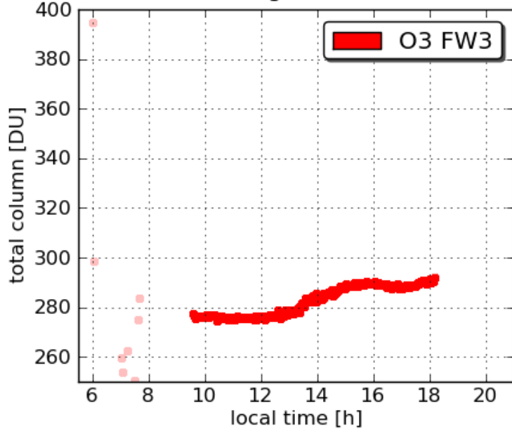
Pandora18 Edgewood 20110718
