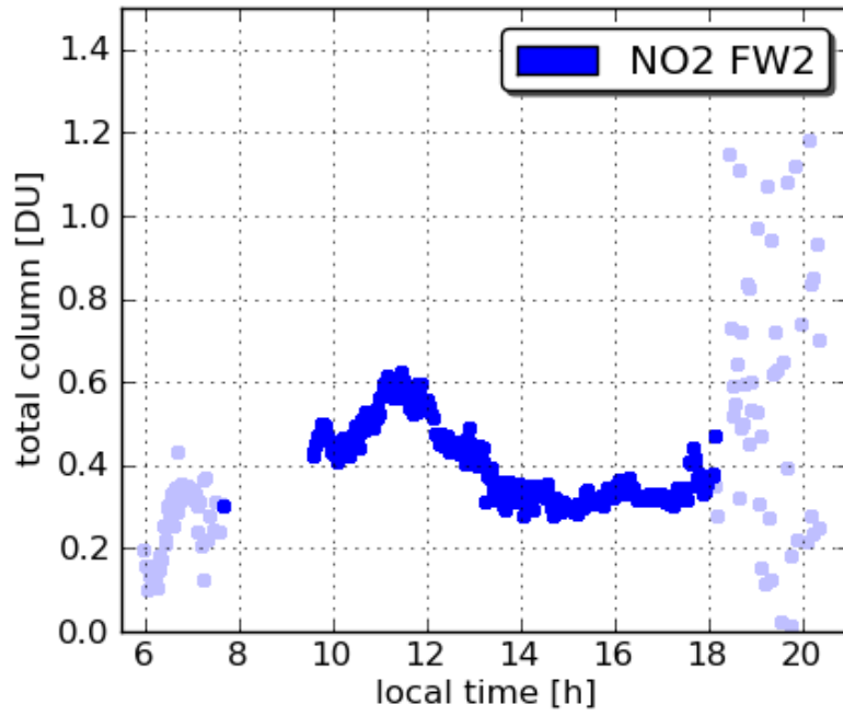
Pandora18 Edgewood 20110718
