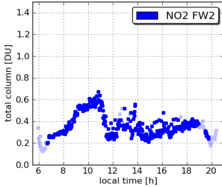
Pandora23 Aldino 20110718
