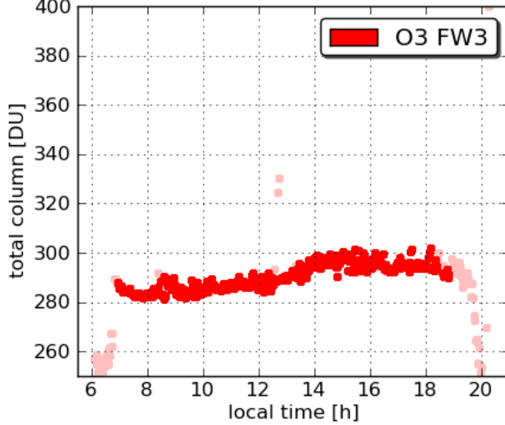
Pandora23 Aldino 20110718
