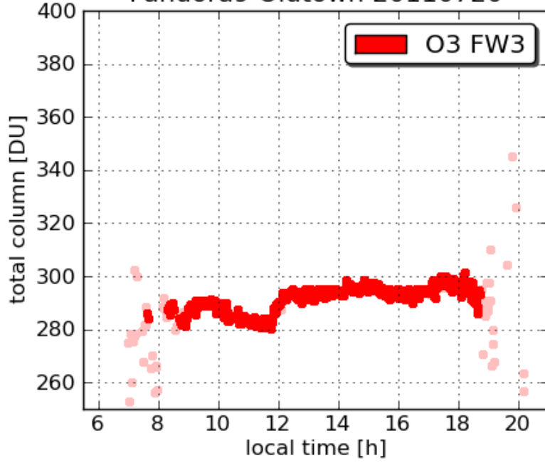
Pandora9 Oldtown 20110720
