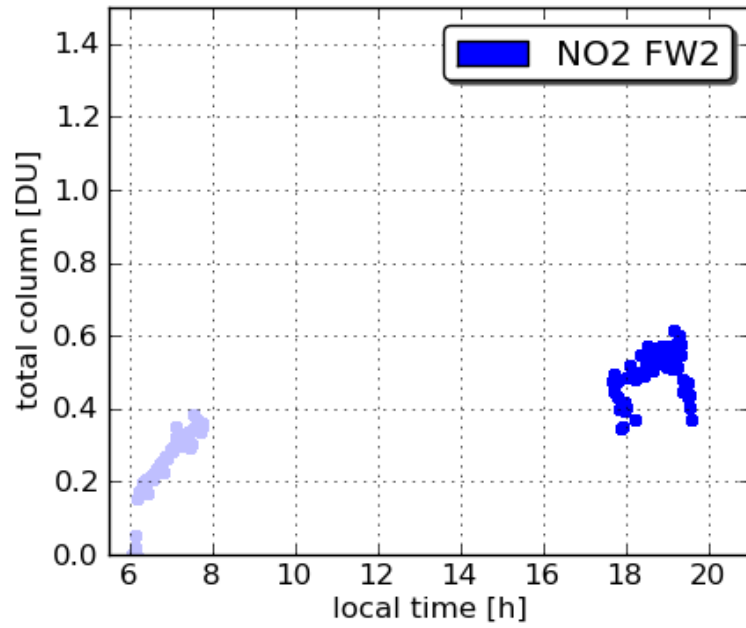
Pandora21 UMCP 20110720
