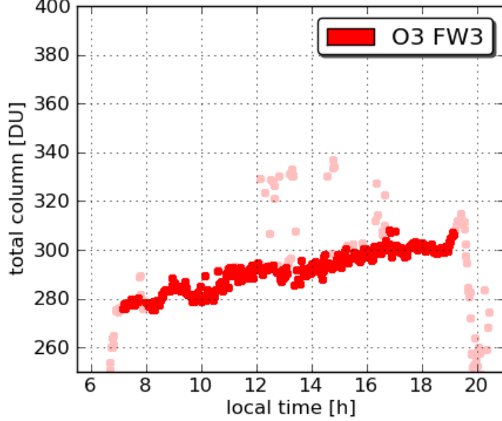
Pandora16 Fairhill 20110720
