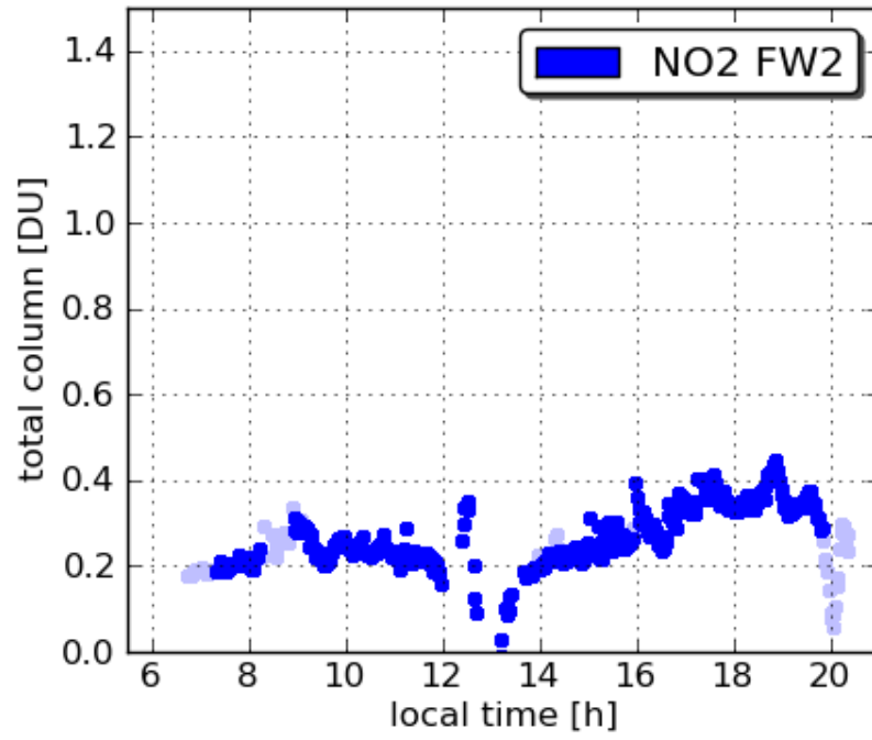
Pandora17 Padonia 20110720
