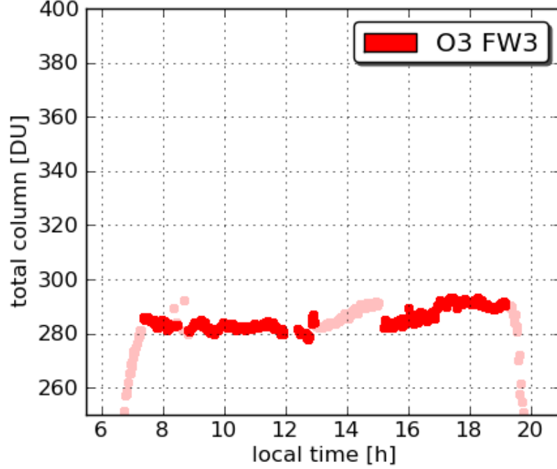
Pandora17 Padonia 20110720
