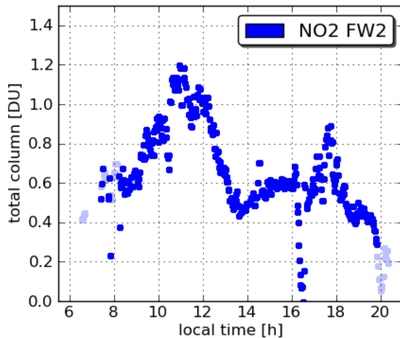
Pandora2 UMBC 20110720
