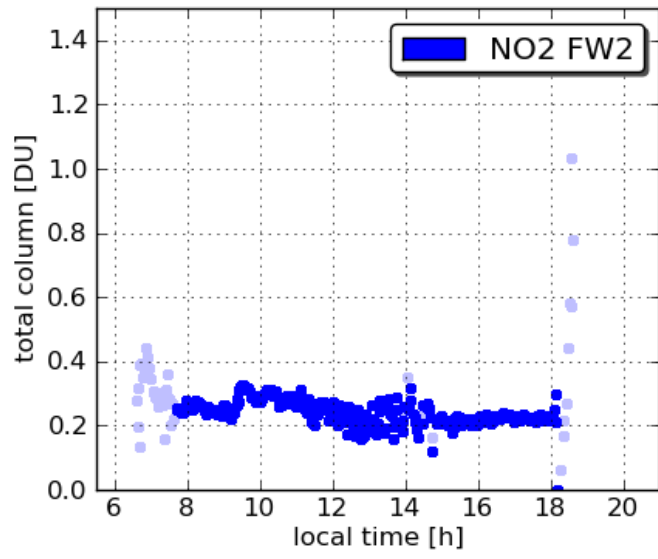
Pandora18 Edgewood 20110720
