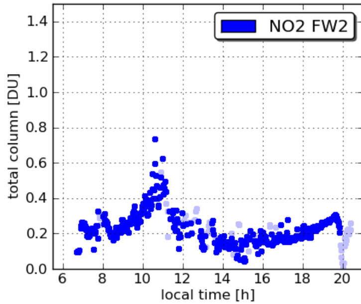
Pandora16 Fairhill 20110720
