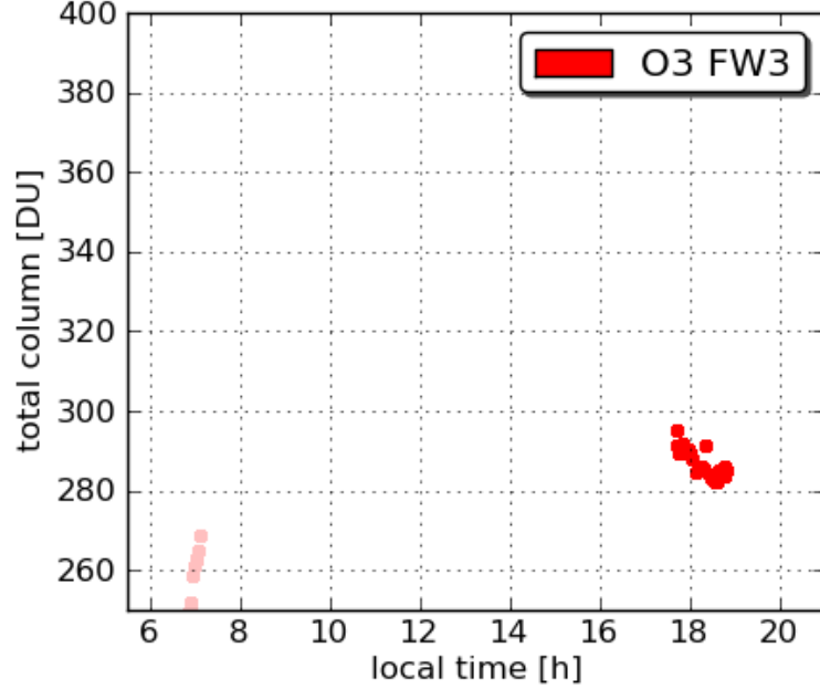
Pandora21 UMCP 20110720
