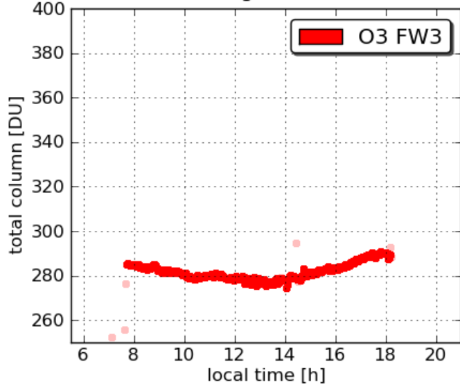
Pandora18 Edgewood 20110720
