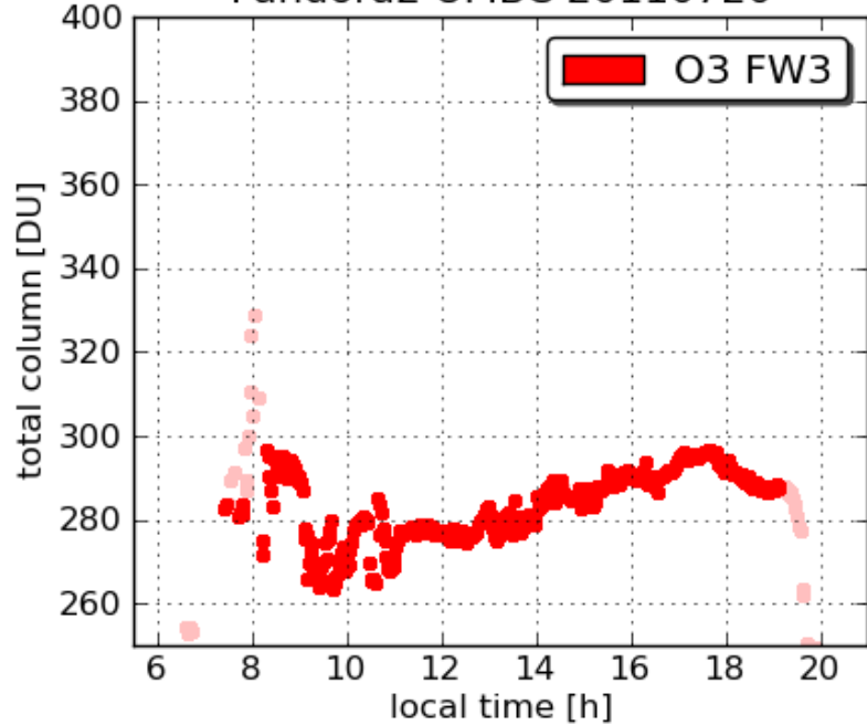
Pandora2 UMBC 20110720
