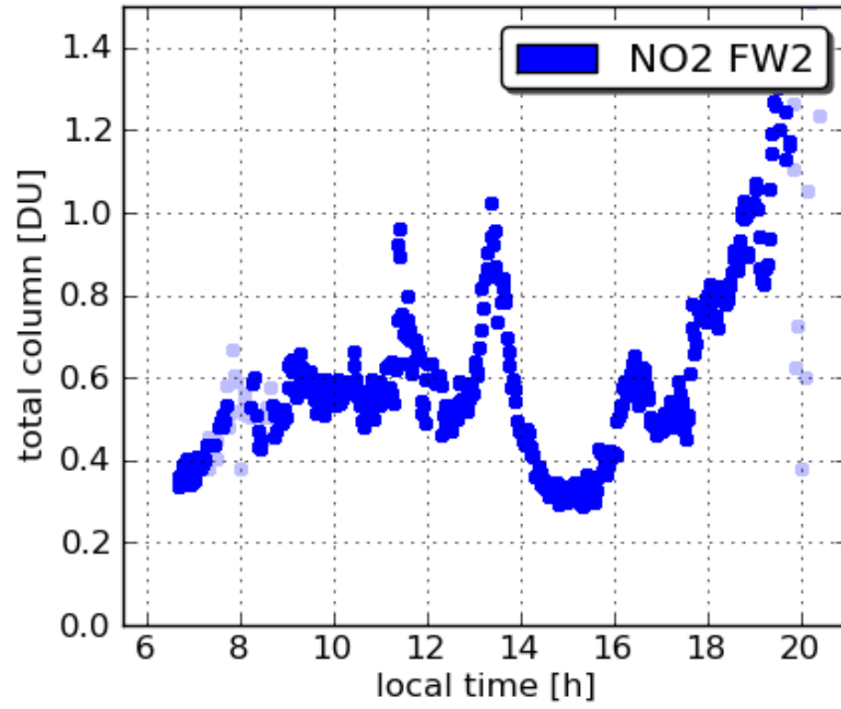
Pandora9 Oldtown 20110720
