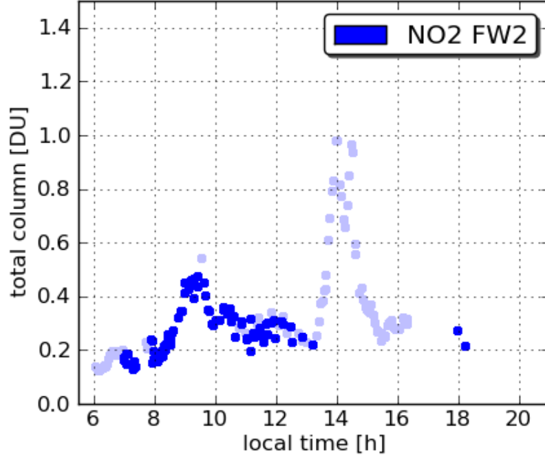
Pandora16 Fairhill 20110725
