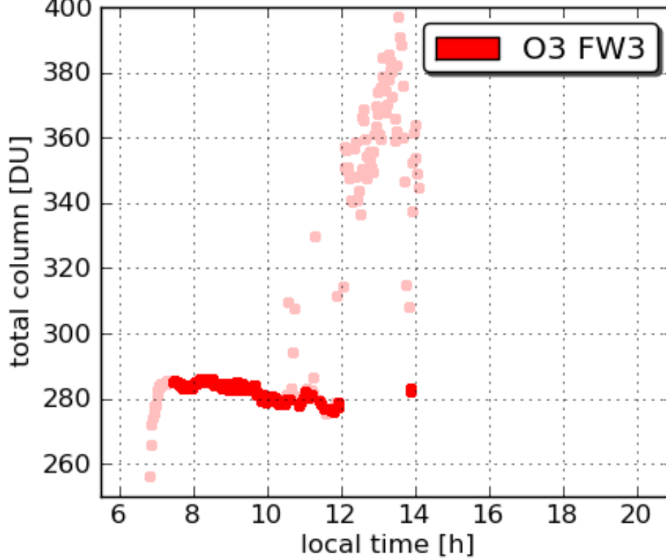
Pandora3 GSFC 20110725
