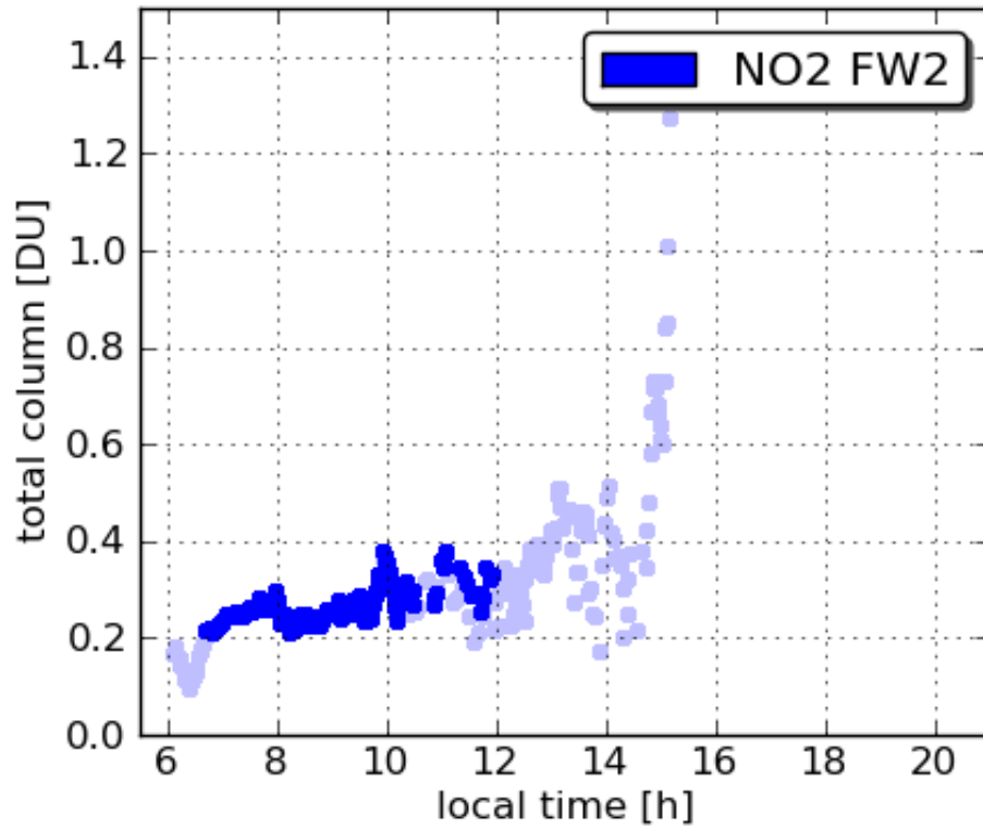
Pandora3 GSFC 20110725
