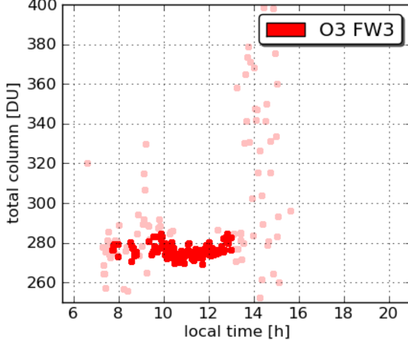
Pandora7 SERC 20110725
