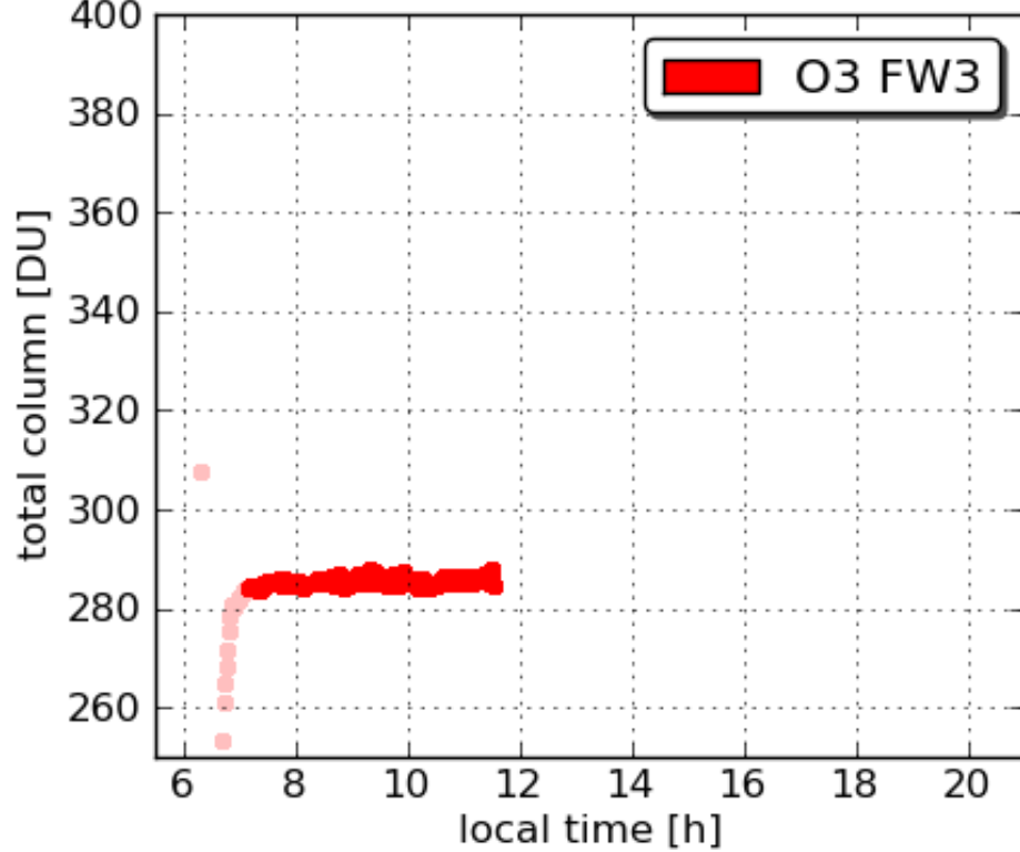
Pandora19 Essex 20110725
