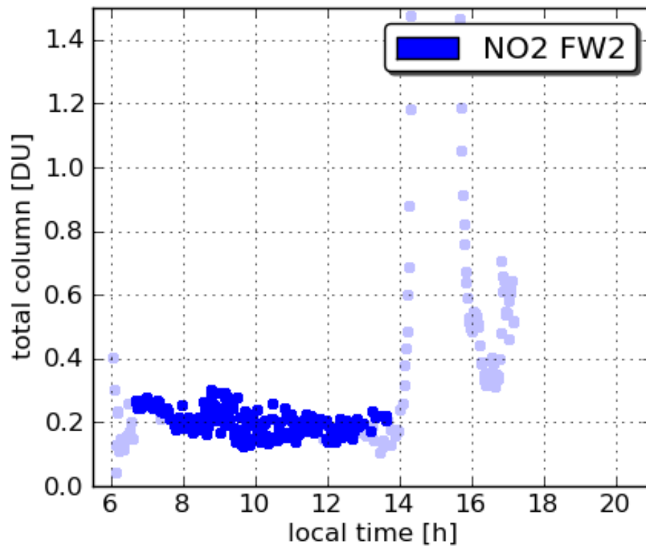
Pandora19 Essex 20110725
