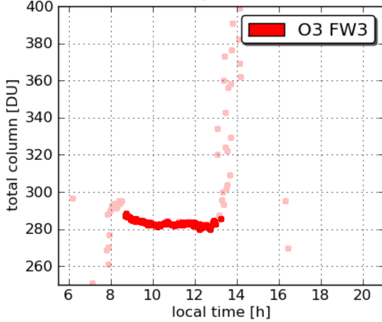
Pandora18 Edgewood 20110725
