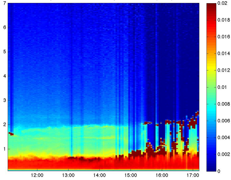
ALS-450 355 nm AttBack 27-Sep-2013 11:03 - 27-Sep-2013 17:12 (UTC)
