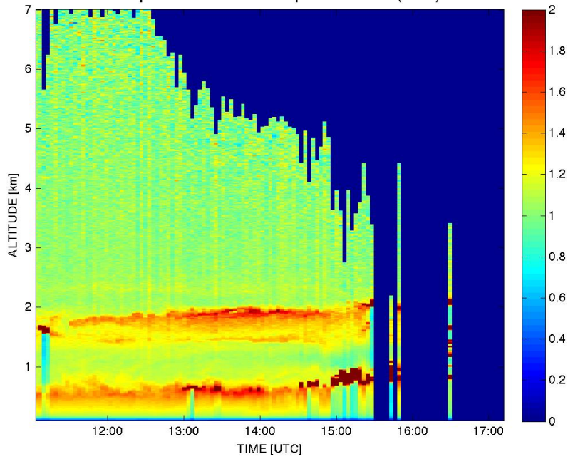
Leosphere ALS-450 355 nm BSR 27-Sep-2013 11:03 - 27-Sep-2013 17:12 (UTC)
